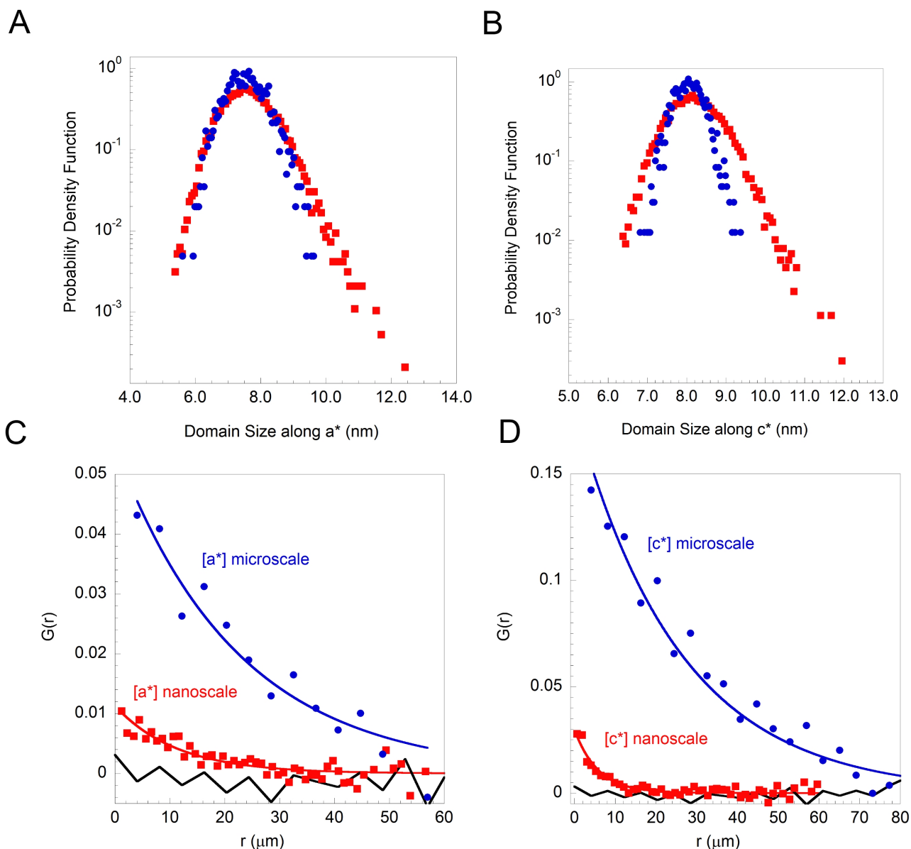
Figure 4 | Probability density function of the domain size along a -axis (A) and along c -axis (B) obtained by the microbeam (filled circles) and the nanobeam (filled squares) measurements. Radial correlation function G(r) calculated on domain size map along a -axis (C) and c -axis (D). The blue circles and the red filled squares correspond to the \mu\text{XRD} and \text{nXRD} measurements. A comparison between the G(r) behaviors is shown.
